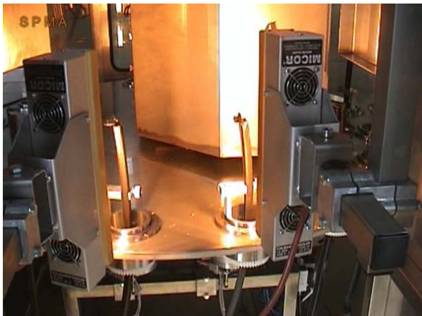
Round table machine with air circulation or infrared dryer
