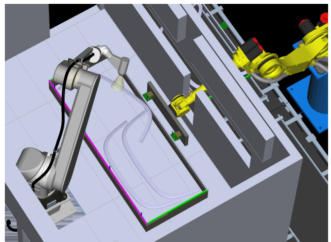
Robotersimulation
